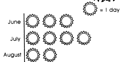
Days with Temperatures Above 100^{\circ} Fahrenheit
